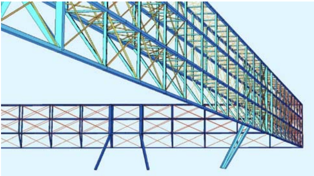
Munich, SWISS-RE Germany, computer model of steel construction
