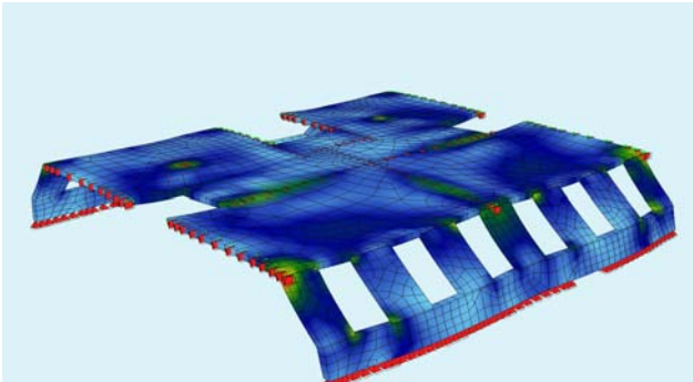
Computer model of spatial concrete roof construction
