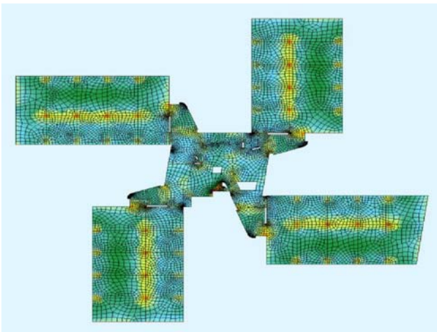
SWISS-RE Germany, computer model of concrete slab with bending stresses
