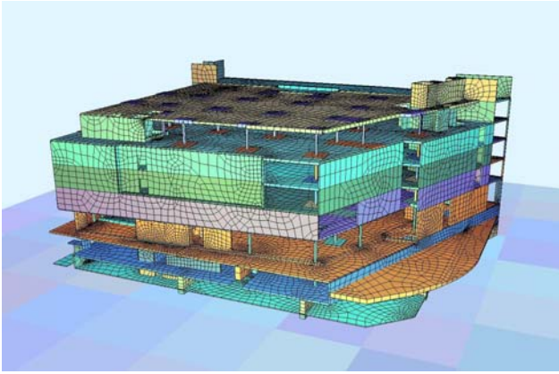
Munich, Karstadt-Oberpollinger, computer model of complete building part C
