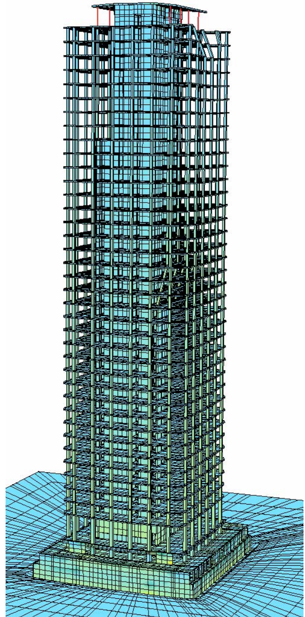
Business tower Uptown Munich, computer model of complete building
